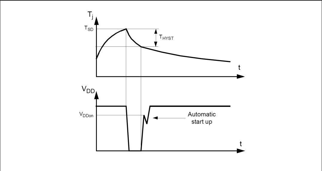
Figure 13. Thermal shutdown
