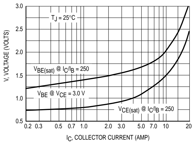
Figure 12. "On" Voltages
