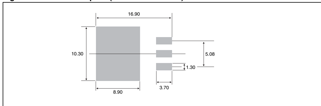
Figure 13. D 2 PAK footprint (dimensions in mm)
