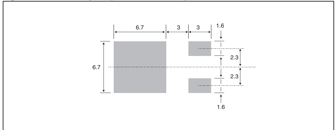
Figure 12. DPAK footprint (dimensions in mm)
