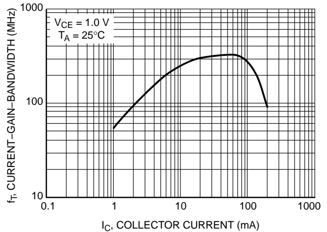
Figure 21. Current-Gain-Bandwidth Product
