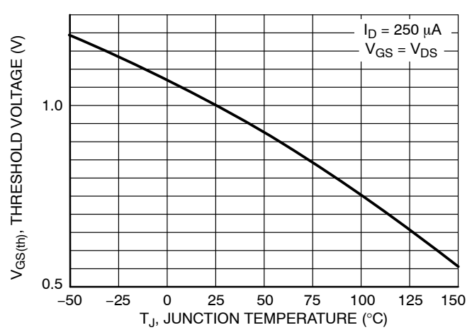
Figure 11. Threshold Voltage
