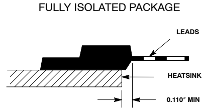
Figure 14. Mounting Position
