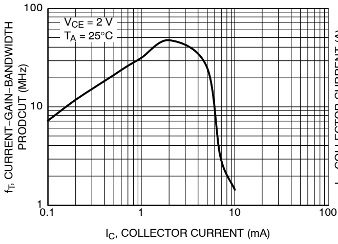
Figure 4. Current-Gain-Bandwidth Product
