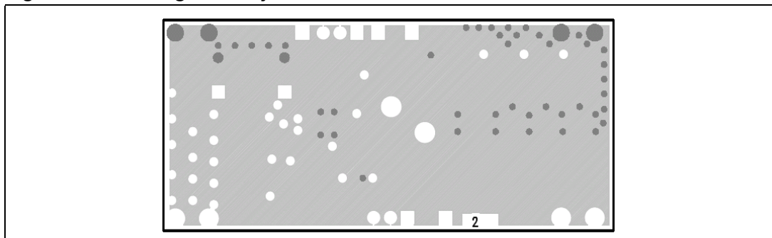
Figure 24. Signal-ground layer
