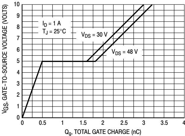
Figure 7. Gate Charge versus Gate-to-Source Voltage
