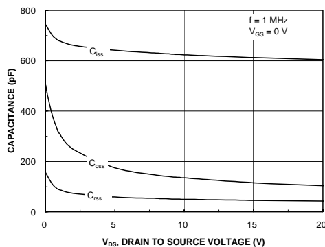
Figure 8. Capacitance Characteristics.
