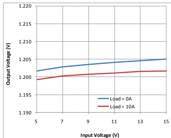
Figure 10. Line Regulation
