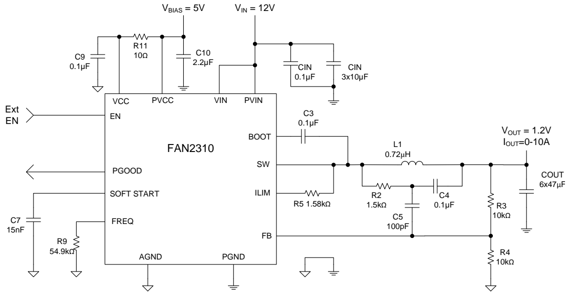
Figure 1. Typical Application
