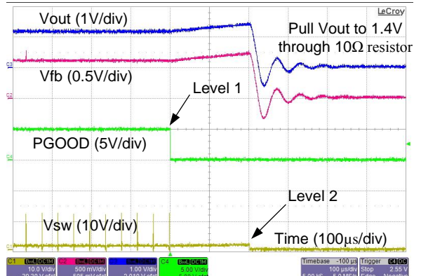
Figure 22. Over-Voltage Protection Level 1 and Level 2
