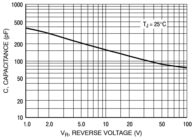
Figure 19. Typical Capacitance
