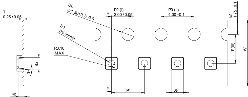
Figure 22. DFN4 1.2 x 1.2 tape and reel
