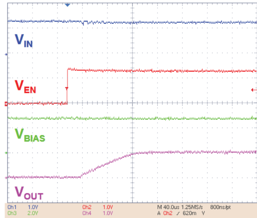
Figure 17. Turn-on time at full load ( I_{OUT} = 500 \text{ mA} ; V_{BIAS} = 2.7 \text{ V} )
