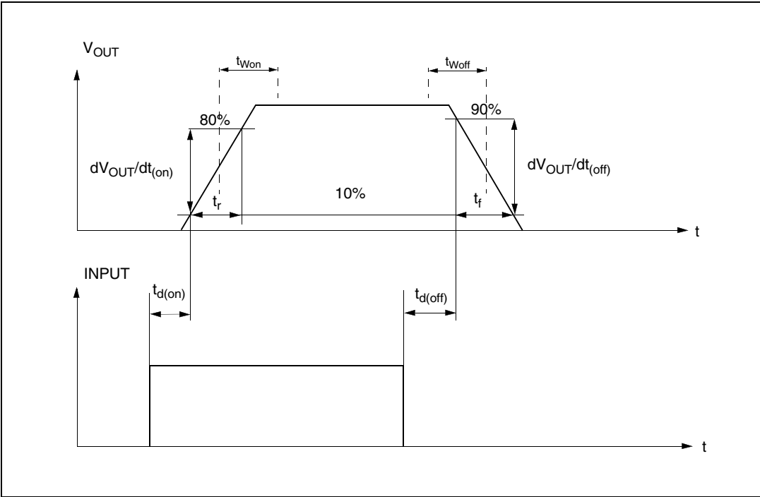
Figure 6. Switching characteristics
