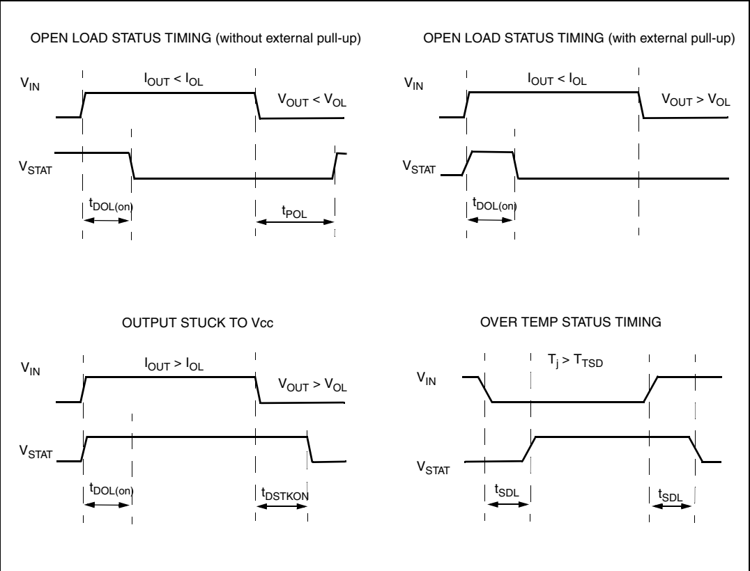
Figure 4. Status timings
