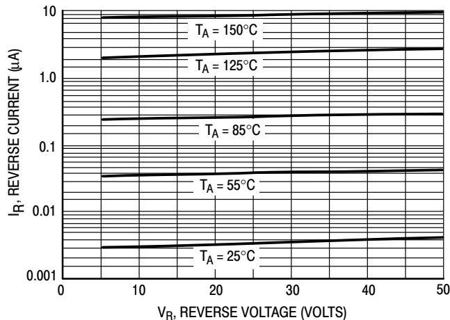
Figure 4. Leakage Current
