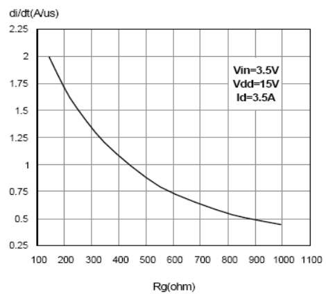
Figure 28. Turn-on current slope ( V_{IN} = 3.5\text{ V} )
