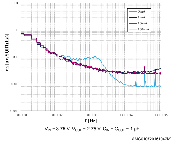
Figure 23. Noise density
