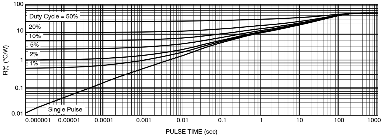
Figure 28. Thermal Response
