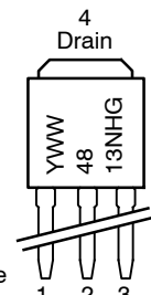
Gate Drain Source
