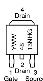
Gate Drain Source
