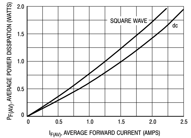
Figure 6. Power Dissipation
