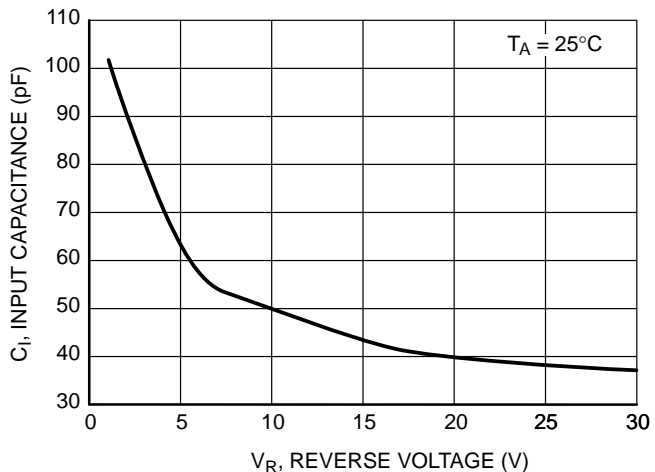
Figure 3. Input Capacitance
