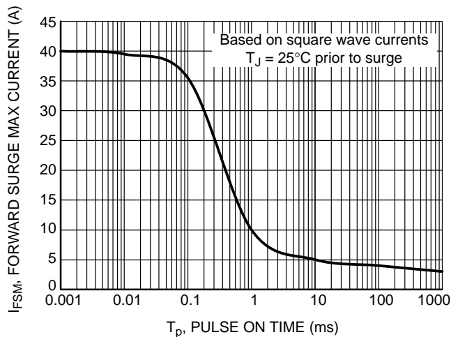
Figure 4. Forward Surge Current
