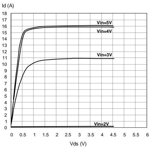
Figure 33. Output Characteristics
