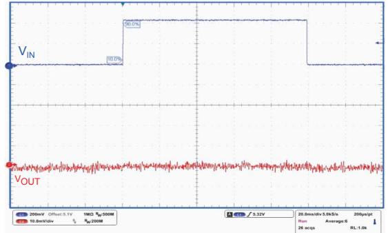
Figure 26. Line transient ( V_{OUT} = 5\text{ V} )
