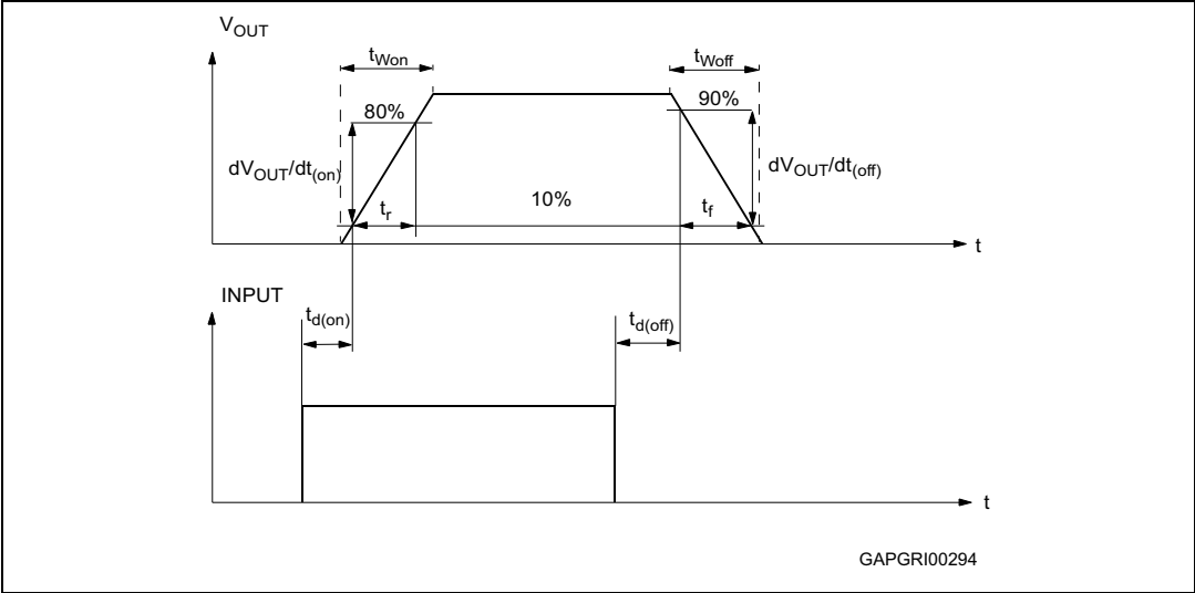
Figure 5. Switching characteristics
