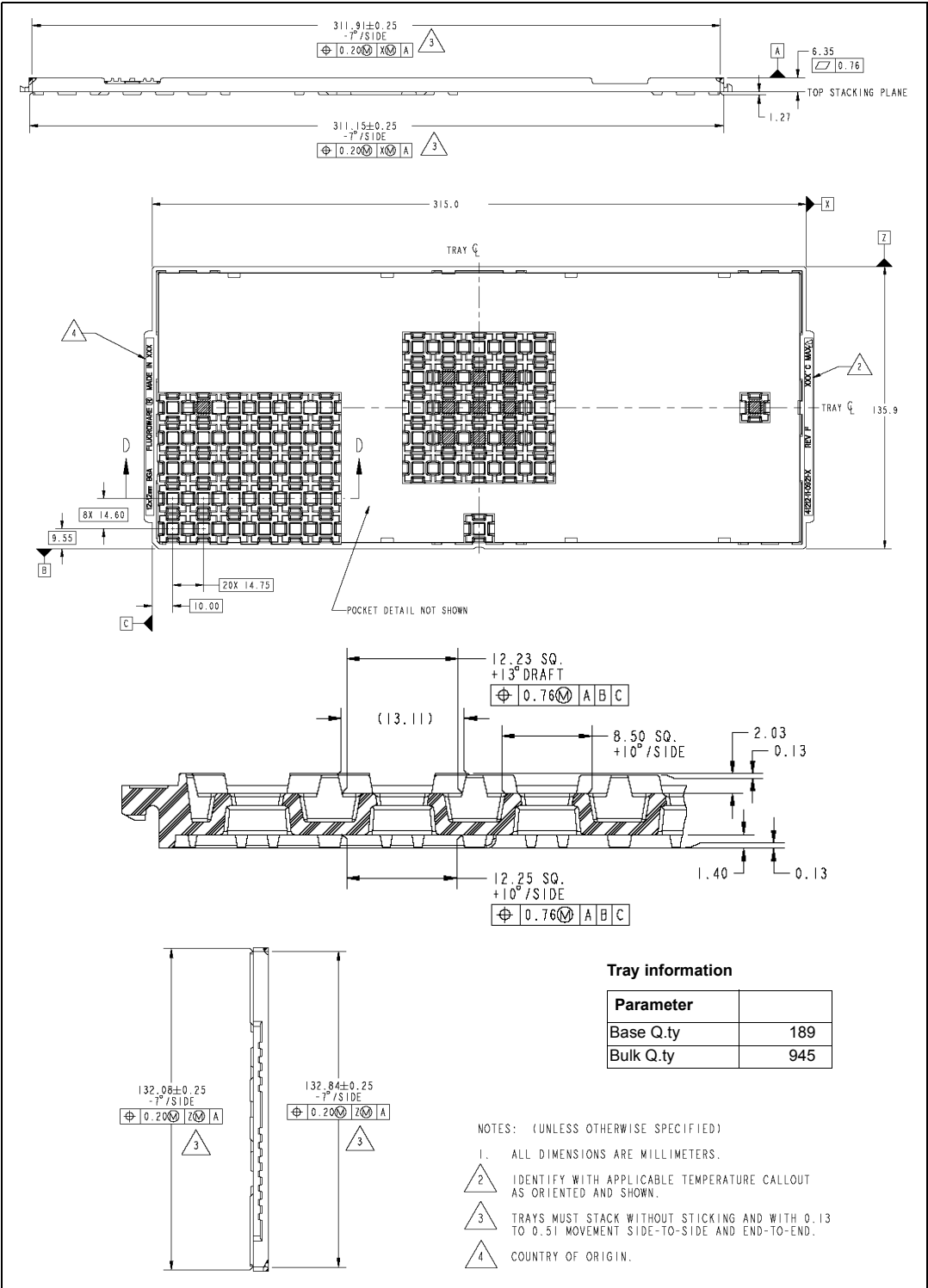
Figure 35. PQFN - 12x12 power lead-less tray shipment (no suffix)
