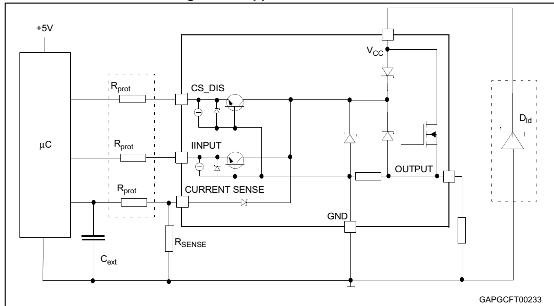
Figure 22. Application schematic
