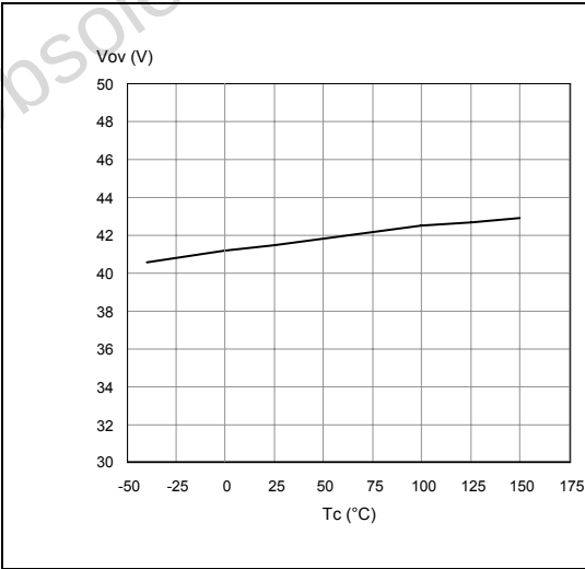
Figure 11. Overvoltage shutdown
