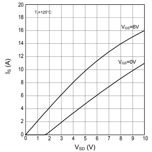
Figure 16. Typ I_{SD\_LS} vs. V_{SD\_LS} at T_J=125^\circ\text{C}
