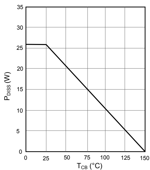
Figure 24. HS Derating curve
