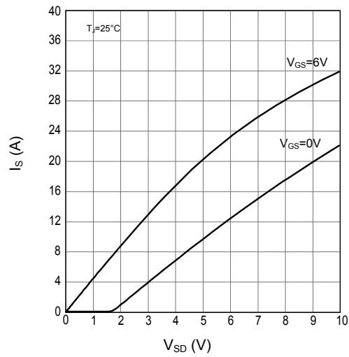
Figure 15. Typ I_{SD\_LS} vs. V_{SD\_LS} at T_J=25^\circ\text{C}
