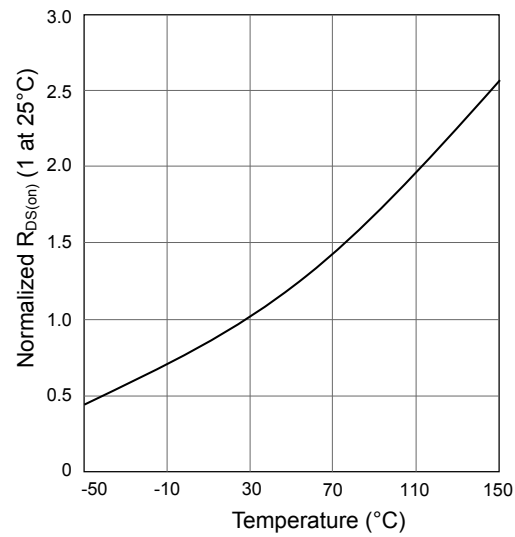
Figure 14. Typ R_{DS(on)} vs. T_J normalized at 25^\circ\text{C}
