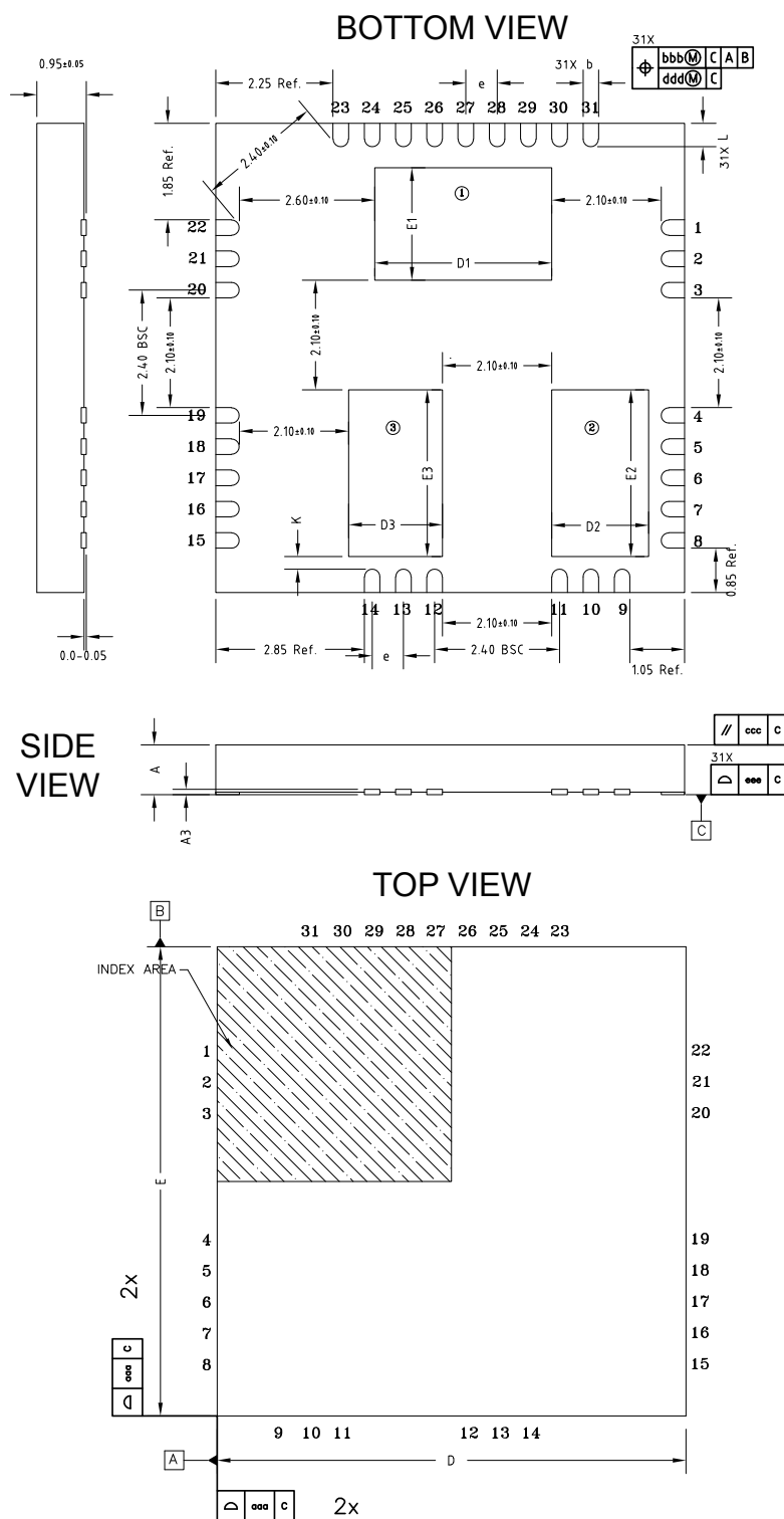
Figure 30. QFN 9 x 9 x 1 mm package dimensions
