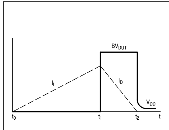
Figure 12. Current-Voltage Waveforms
