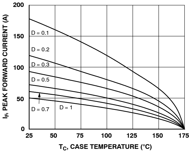
Figure 3. Current Derating
