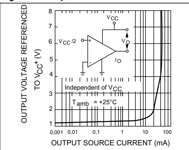
Figure 8. Output characteristics
