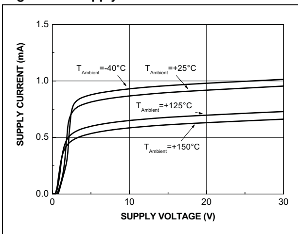
Figure 7. Supply current
