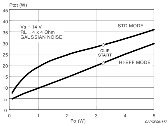
Figure 17. Power dissipation vs. average output power (audio program simulation, 4 \Omega )
