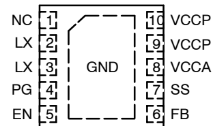
NCP1593A (Top View)
