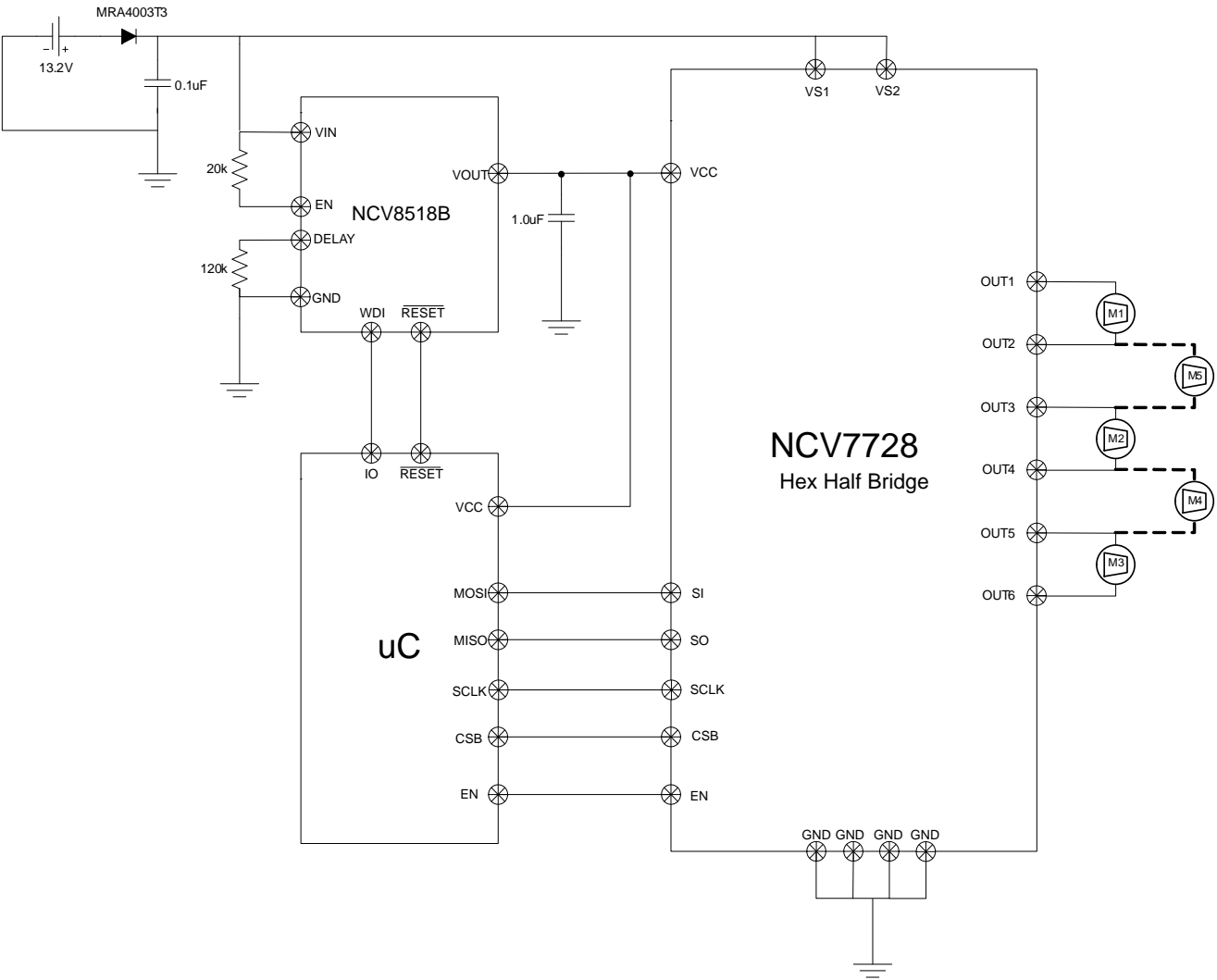
Figure 29. Application Drawing
