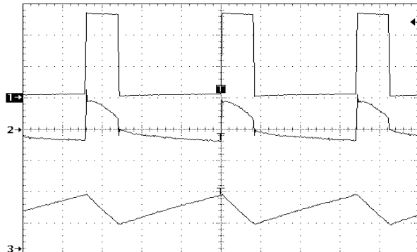
Figure 41. NCP1402SN30T1 Operating Waveforms (Medium Load)
