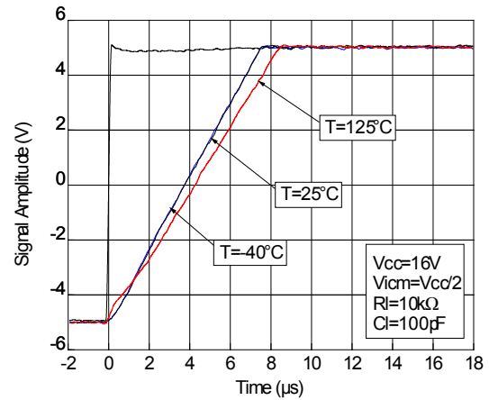
Figure 13. Positive slew rate at V CC = 16 V
