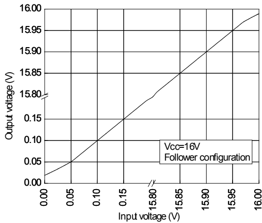
Figure 10. Output voltage vs. input voltage close to the rail at V CC = 16 V
