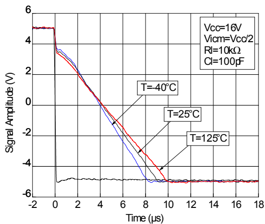
Figure 12. Negative slew rate at V CC = 16 V
