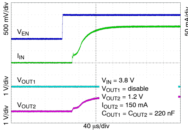
Figure 34. Enable Turn-on Response - VR1 = Off, VR2 = 150 mA
