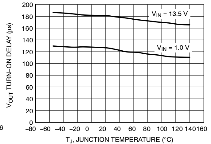
Figure 14. Output Turn-on Delay vs. Temperature
