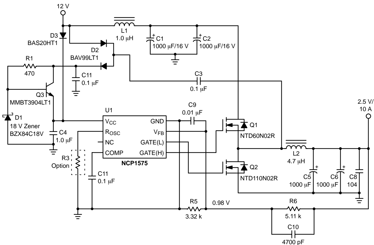
Figure 1. 12 V Only Applications Diagram, 12 V to 2.5 V Conversion at 10 A
