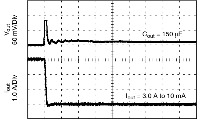
Figure 10. Load Transient Response
