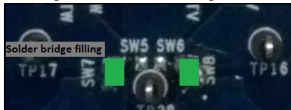
Figure 11: Three-shunt configuration
