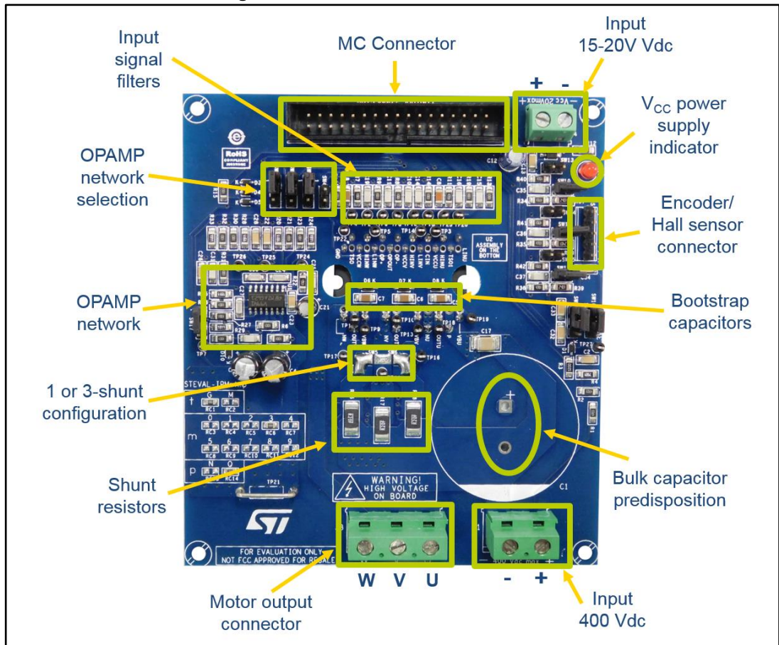
Figure 8: STEVAL-IPMnM1N architecture
