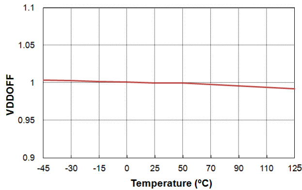
Figure 18. VDDOFF vs. Temperature
