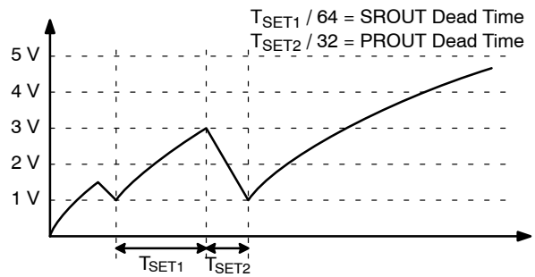
Figure 73. Multi-function Operation of RDT Pin
