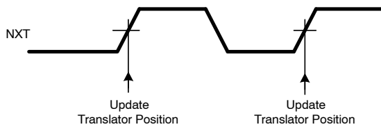
Figure 11. Translator Position Timing Diagram
