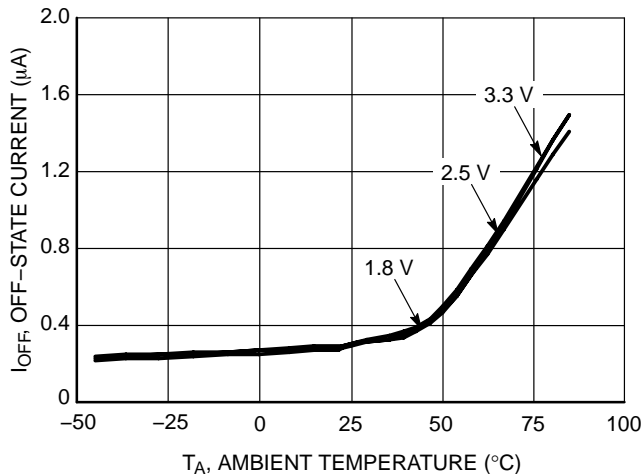
Figure 29. Off-Stage Current versus Ambient Temperature
