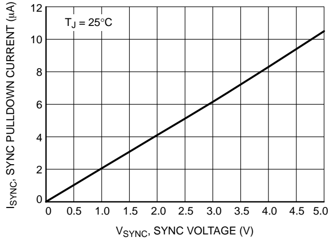
Figure 4. Sync Pulldown Current vs. Sync
