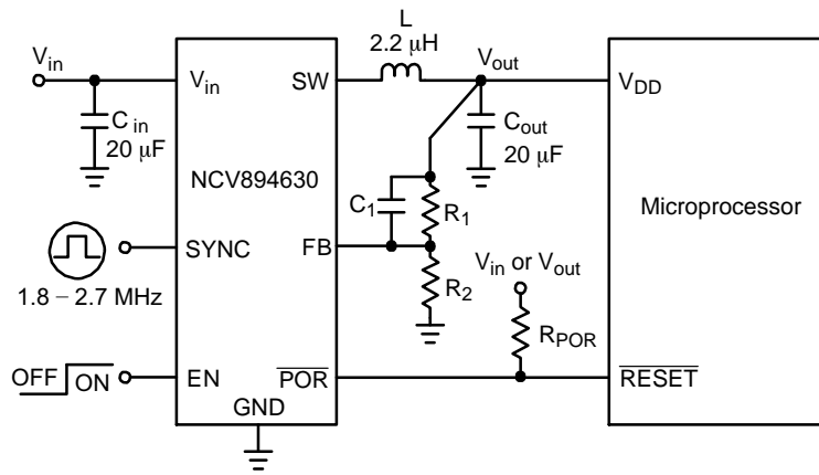
Figure 1. NCV894630 Typical Application
