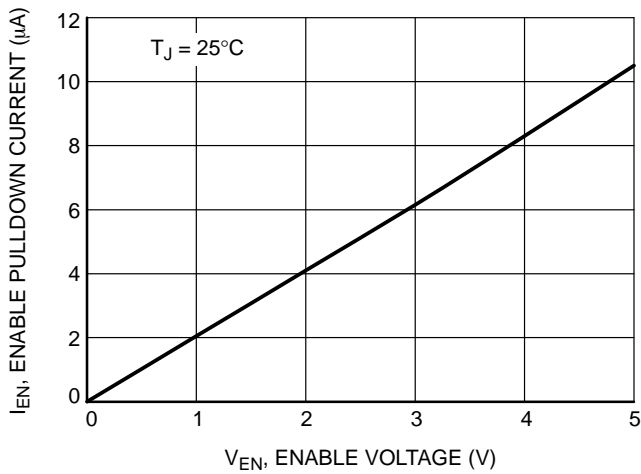
Figure 5. Enable Pulldown Current vs. Enable
