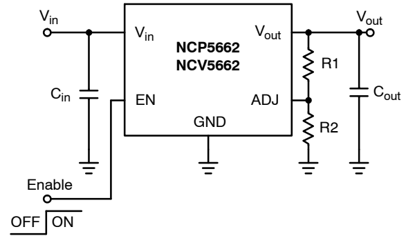
Figure 2. Typical Application Schematic, Adjustable Output
