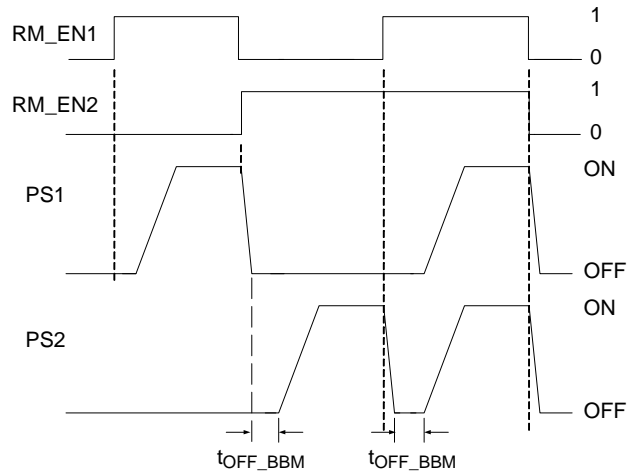
Figure 6. Break-Before-Make Switching
