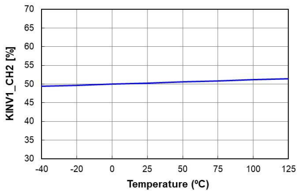
Figure 26. K INV1-CH2 vs. Temperature
