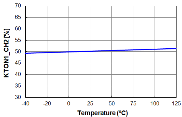
Figure 24. K TON1-CH2 vs. Temperature
