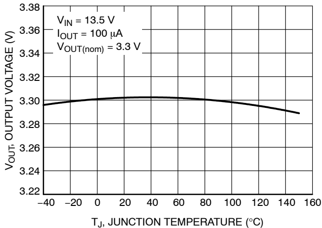
Figure 17. Output Voltage vs. Junction Temperature
