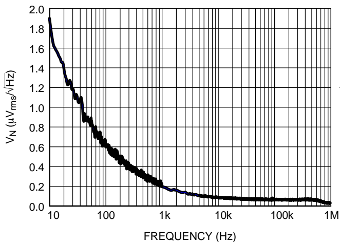
Figure 21. Output Noise vs. Frequency, 0.7 V Version
