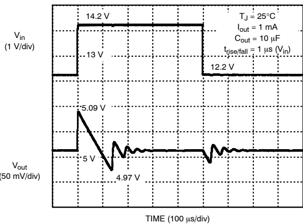
Figure 16. Line Transients
