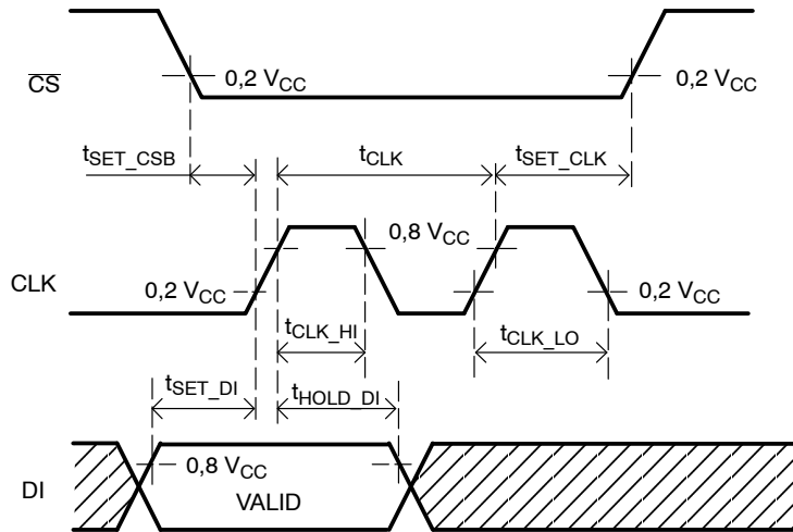
Figure 5. SPI Timing
